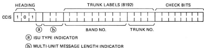
Fig. 8—Initial Signal Unit (ISU) format.
