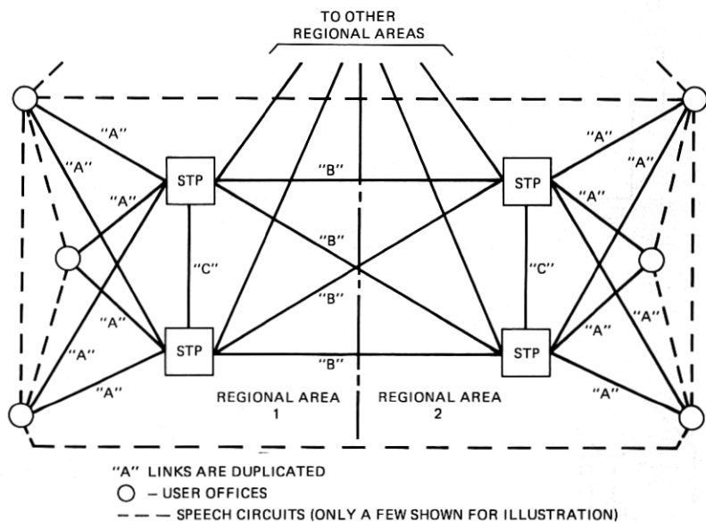
Fig. 3—User offices connected to STP quad.
