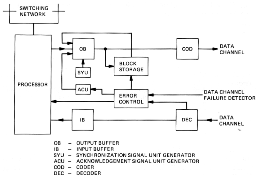
Fig. 6—Functional block diagram of a CCIS terminal.
